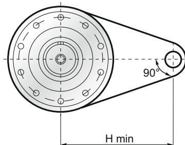
Figure 10: Torque Arm
