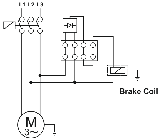
Figure 13: Standard Type Brake Anchorage Schema
