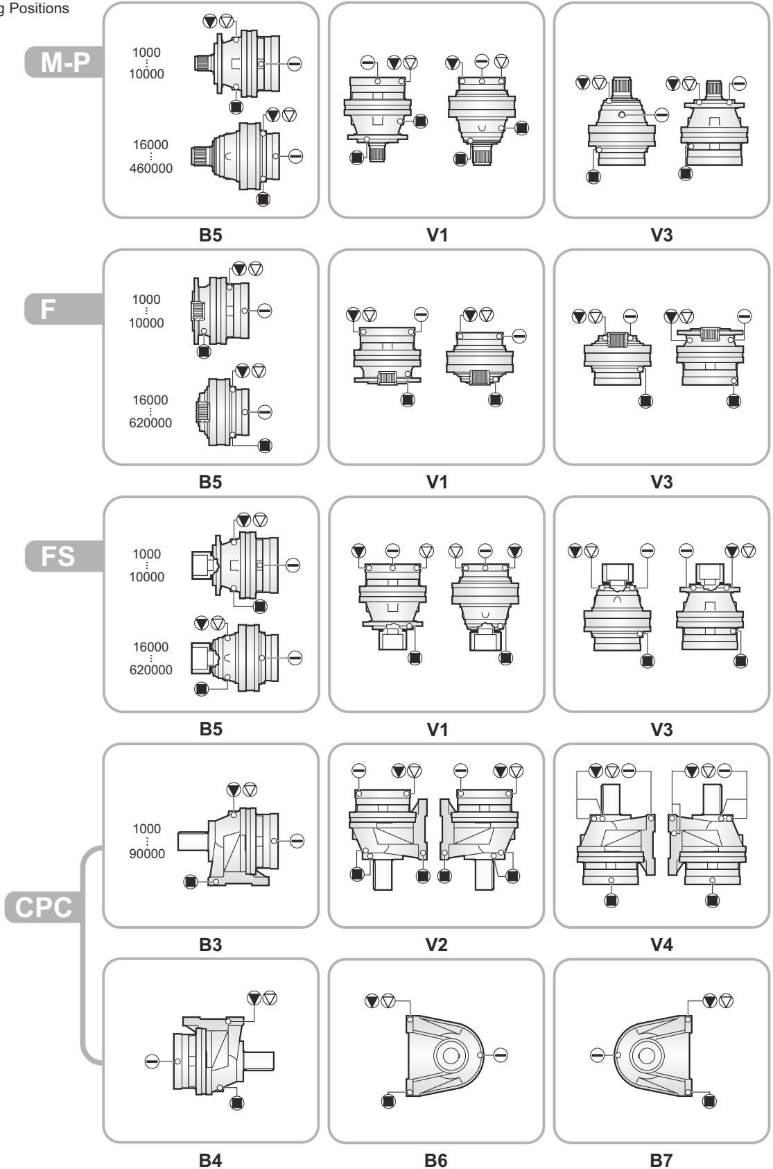
Figure 7: Mounting Positions
