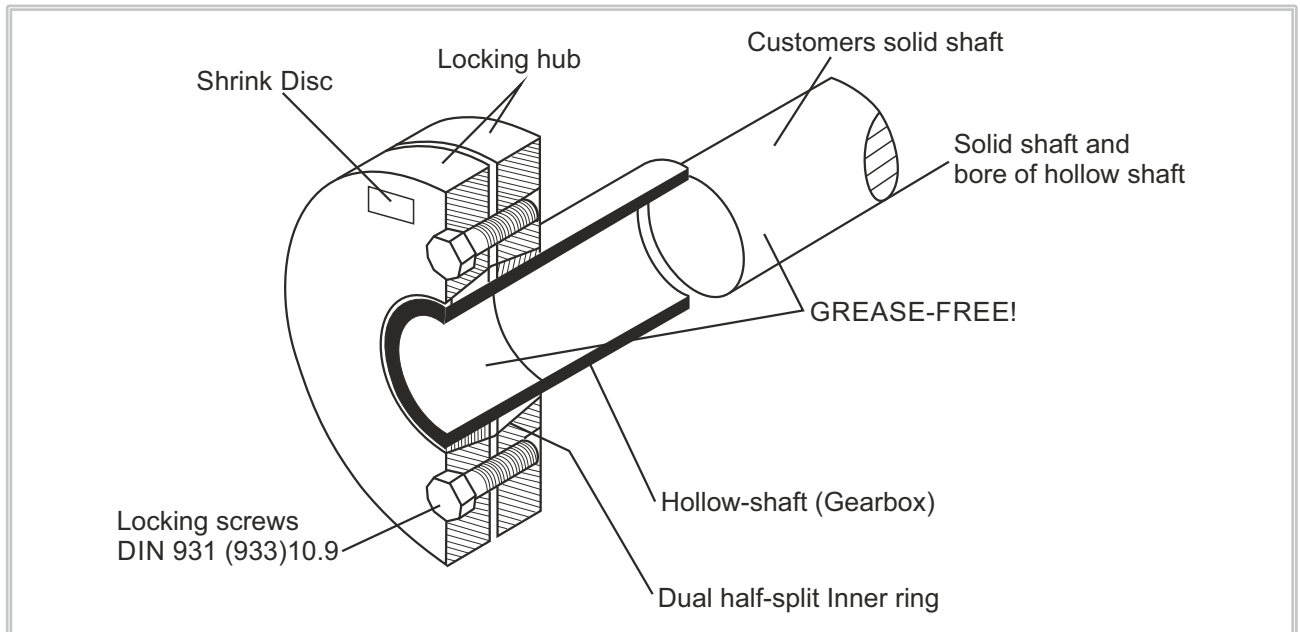
Figure 12: Shrink Disc
