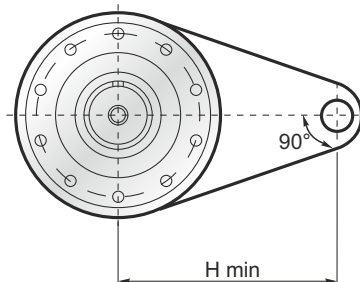
Figure 13: Torque Arm
