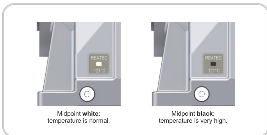
Figure 9: Temperature Sticker 2
