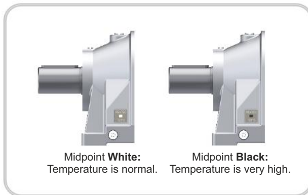
Figure 5: Temperature Sticker 1
