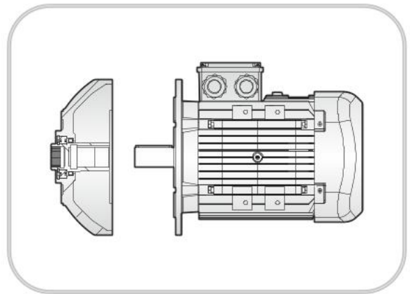
Figure 7: The Mountage of the Standard B5 Motor to the PAM Gear Unit
