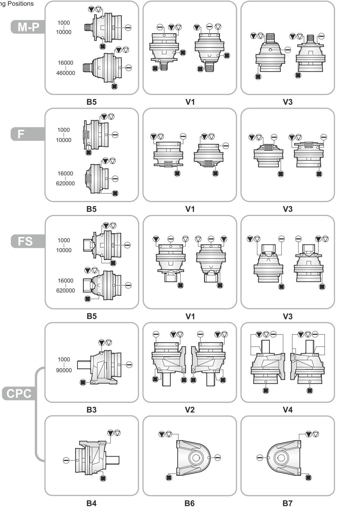
Figure 10: Mounting Positions
